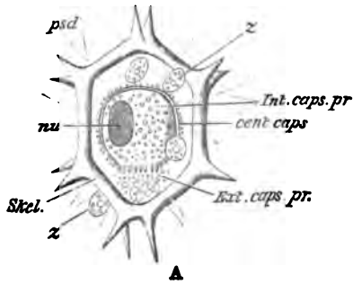
FIG. 26.—A, Lithocercus annularis , with sagittal ring (from Parker and Haswell). B, Aulactinium actinastrum . C, calymma; cent. caps., kn, central capsule; Ext. caps. pr., Extracapsular, and Int. caps. pr., intracapsular protoplasm; n, nu, nucleus; op, operculum; ph, phaeodium; psd, pseudopodium; Skel., skeleton; z, Zooxanthella. (From Lang's Comparative Anatomy , after Haeckel.)
